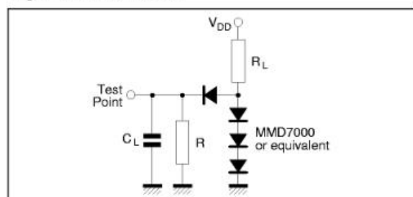
Figure 1 : Test Load
